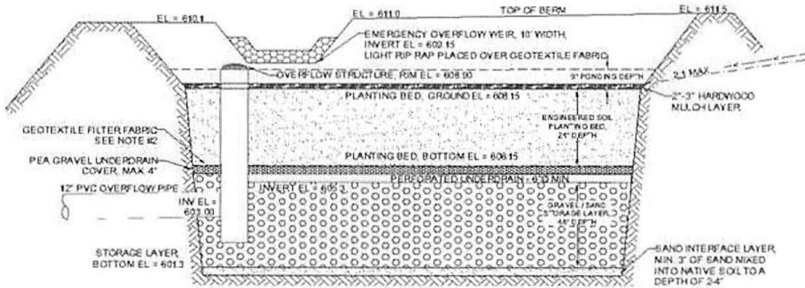
BIORETENTION CELL #1
