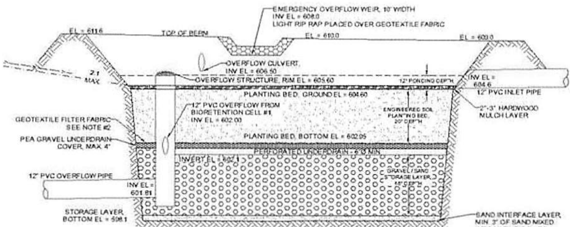
BIORETENTION CELL #2
