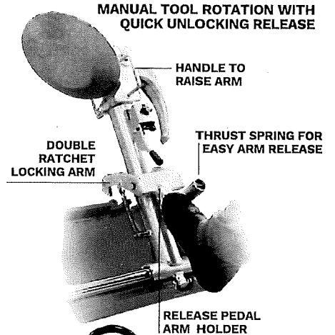
SERVICE TUBE and TUBELESS TIRES The tool operates between bead and rim and demounts the tire.
