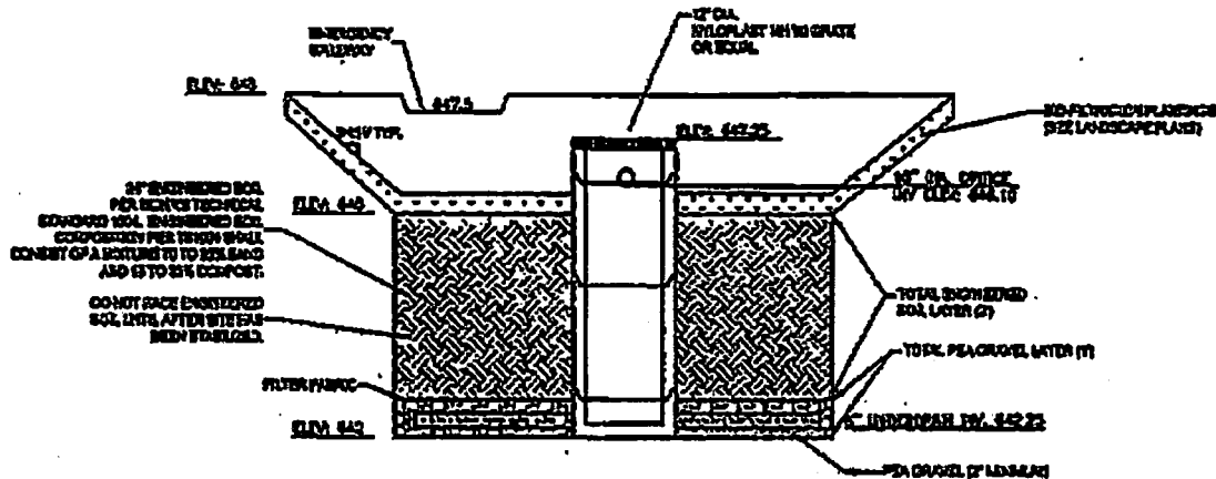
BASIN B (BIO-FILTRATION)
