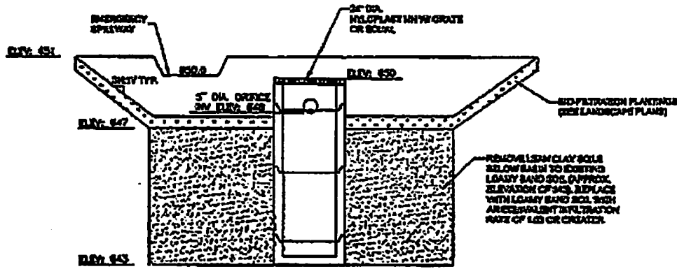
BASIN A (INFILTRATION)
