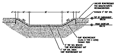
A4 EMERGENCY OVERFLOW WEIR DETAIL N/S
