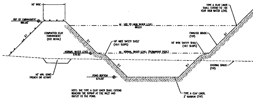
C4 STORMWATER POND CROSS SECTION DETAIL N/S
