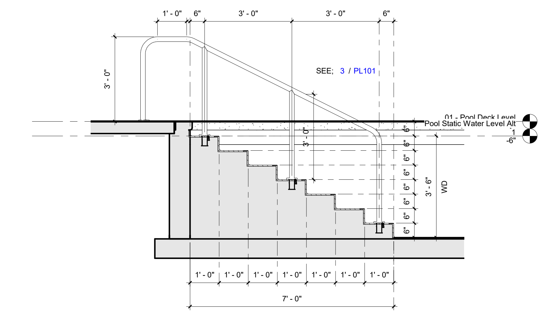
4 POOL A - WARMING POOL STAIRS SECTION VIEW 1/2" = 1'-0"
