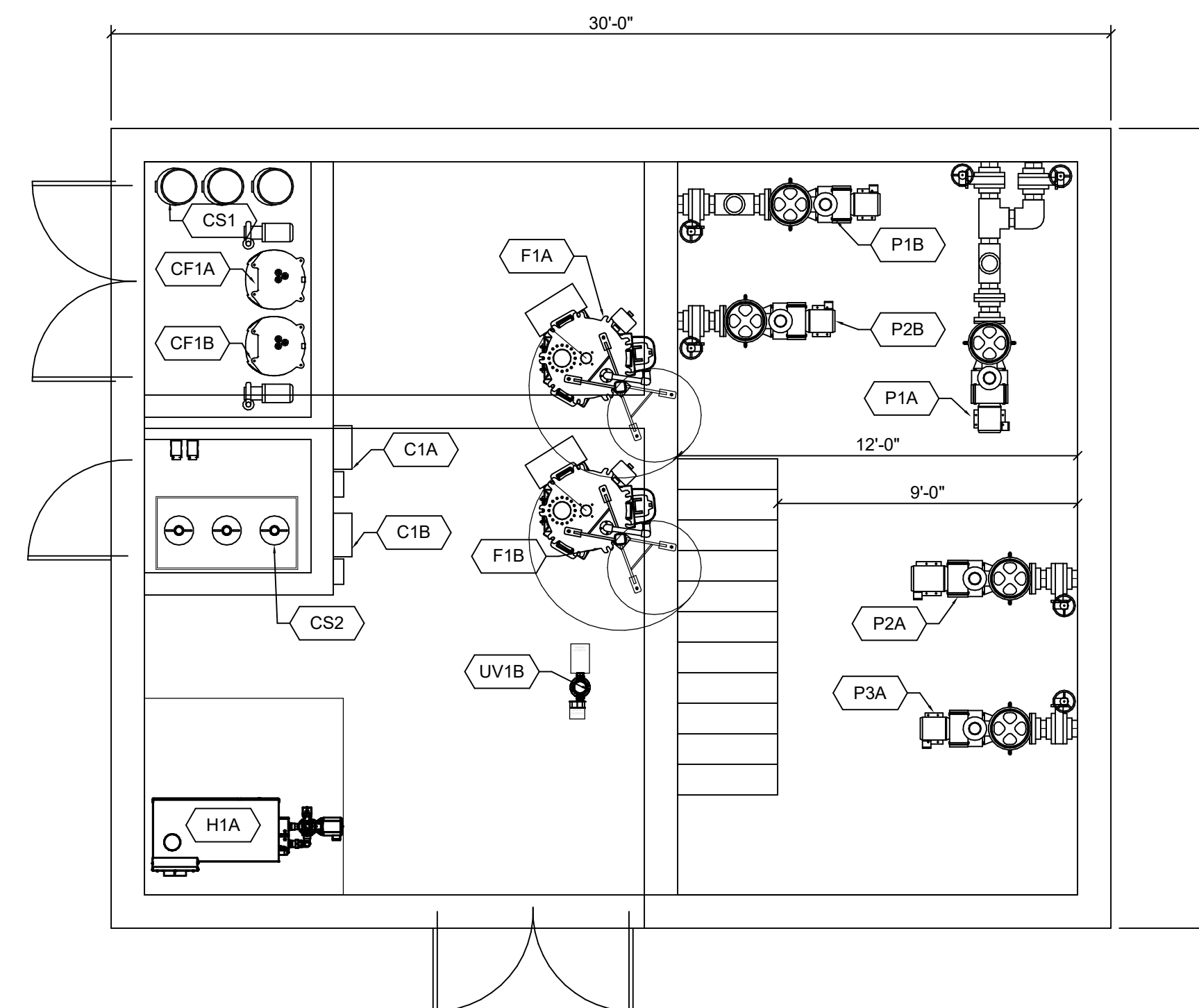
1.1 ALT 2 MECHANICAL ROOM DEFENDER PLAN VIEW 1/4" = 1'-0"
