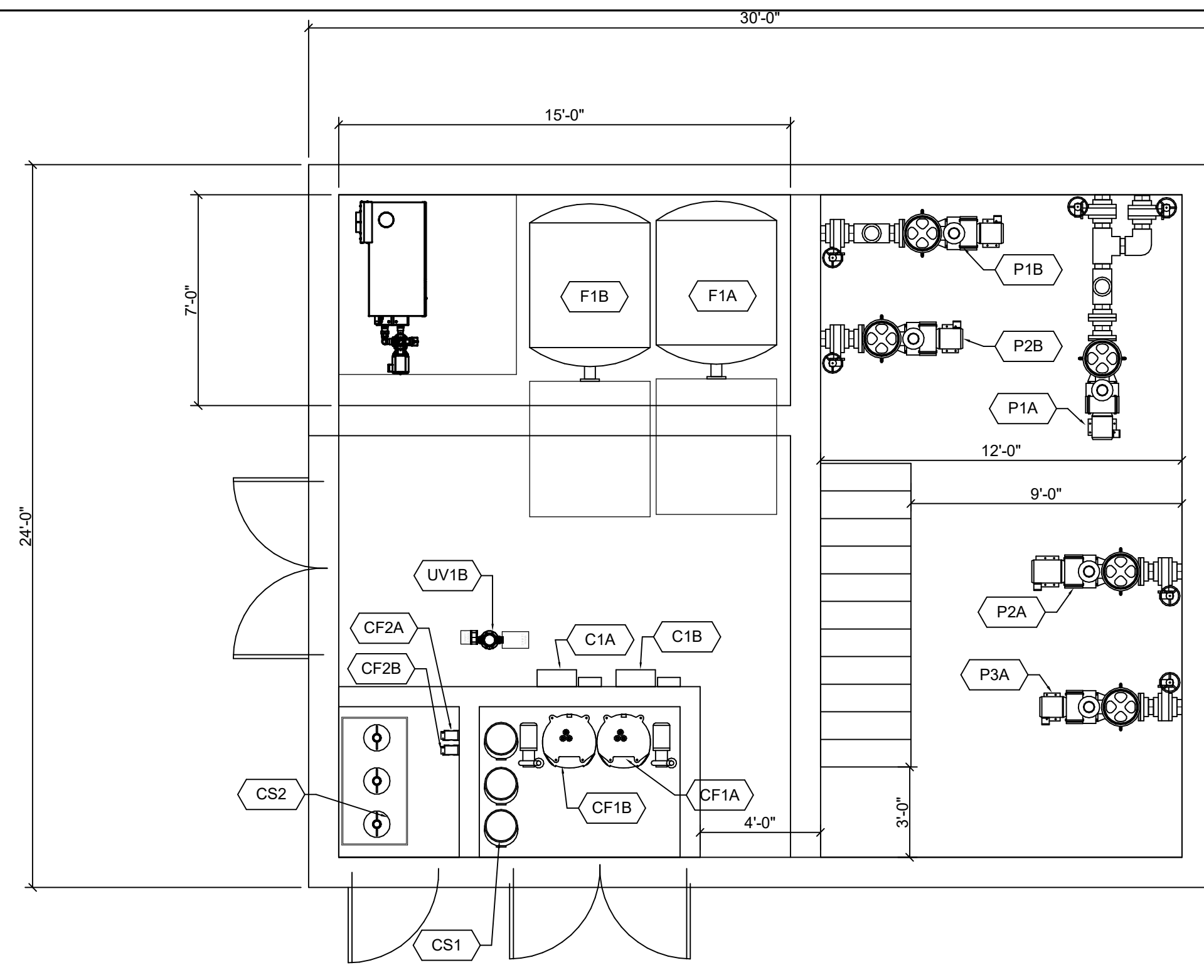
4.1 ALT 2 MECHANICAL ROOM SAND PLAN VIEW 1/4" = 1'-0"
