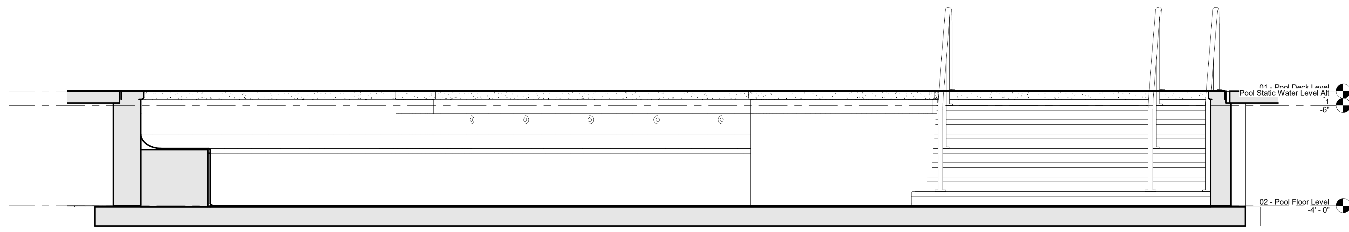
2 POOL B - WARMING POOL SECTION VIEW 1/2" = 1'-0"
