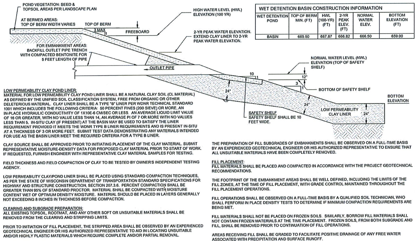
A WET BASIN CROSS SECTION SCALE: 1" = 1'
