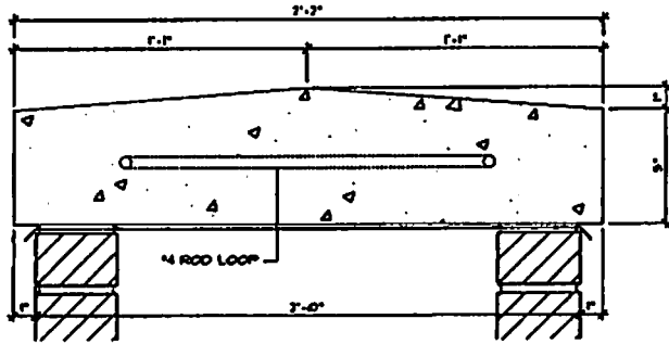
13 CONCRETE PIER CAP DETAIL 7'-2" x 1'-0"
