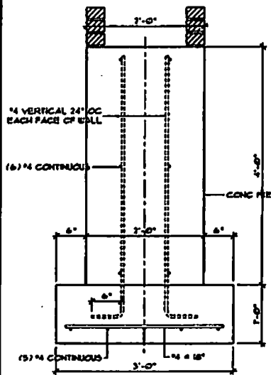
9 FOUNDATION SECTION 7'-0" x 7'-0"
