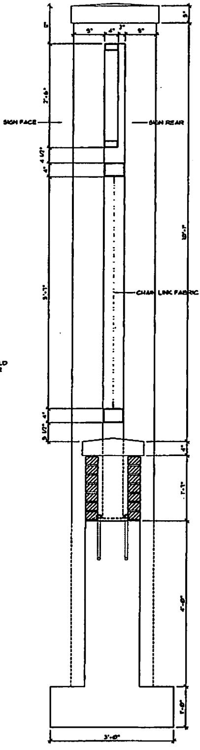
7 SECTION THROUGH SIGN 7'-6" x 7'-0"
