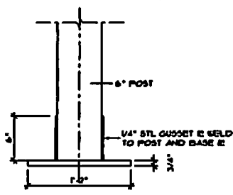
10 BASE PLATE DETAIL 1'-0" x 7'-0"
