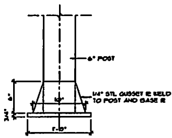
11 BASE PLATE DETAIL 1'-0" x 7'-0"
