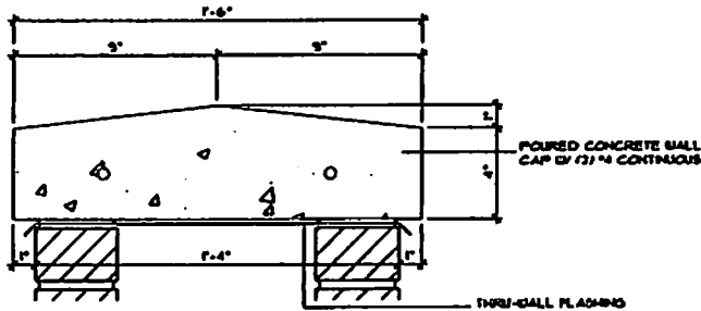
12 CONCRETE WALL CAP DETAIL 7'-6" x 1'-0"
