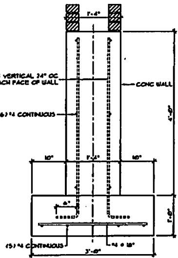
8 FOUNDATION SECTION 7'-6" x 7'-0"
