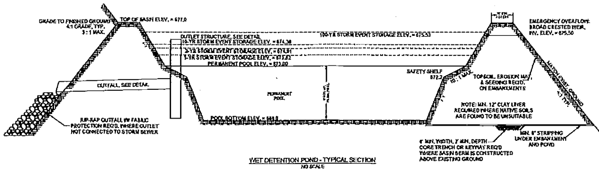
WET DETENTION POND - TYPICAL SECTION NO SCALE
