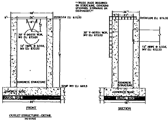
OUTLET STRUCTURE - DETAIL NO SCALE
